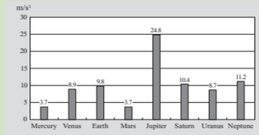
Planet's Gravitational Pulls
